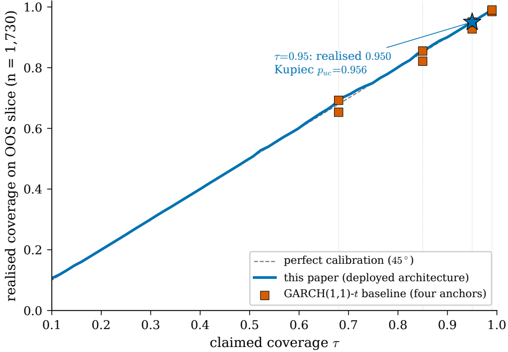
Figure 4: Calibration curves on the 1,730-row 2023+ OOS slice. The deployed architecture (this paper, blue) tracks the 45° diagonal across the served range \tau \in [0.68, 0.99] ; GARCH(1,1)- t markers (vermilion squares) at the four served anchors are the practitioner-standard parametric baseline and visibly under-cover at \tau \in \{0.68, 0.85, 0.95\} (Kupiec figures in §6.4.3). Star marks the headline \tau = 0.95 result.
