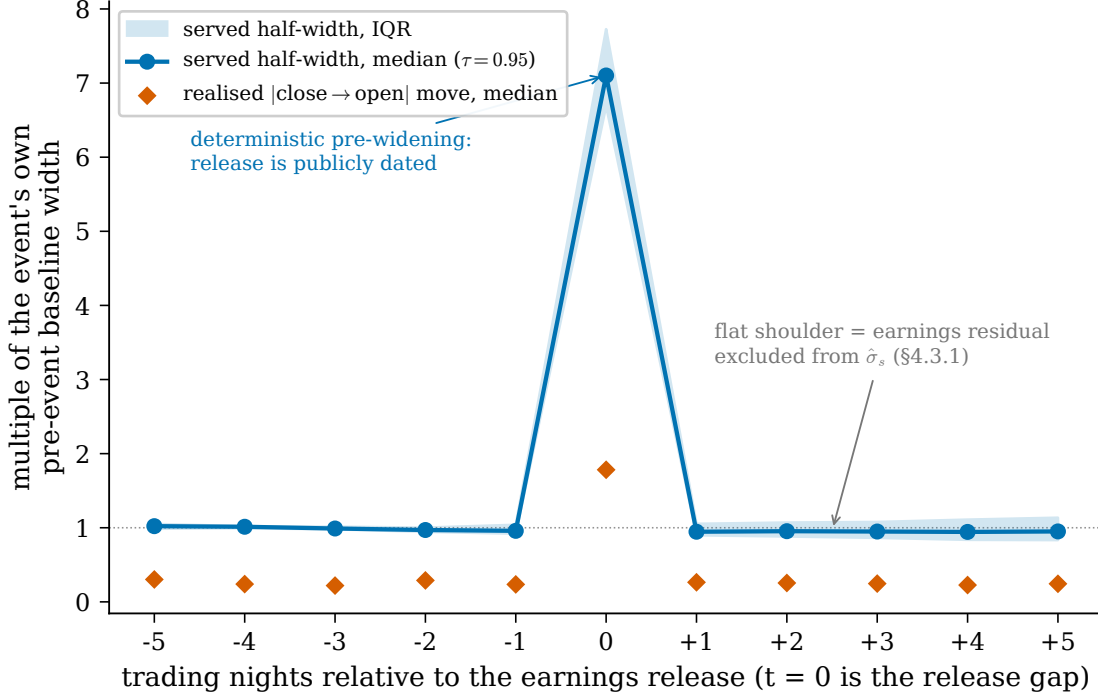
Figure 2: Calendar-conditioned widening in event time: all 228 earnings nights on the overnight panel aligned at t = 0 , each event’s served \tau = 0.95 half-width (deployed artefact schedules) at night offsets t - 5 \dots t + 5 normalised by that event’s own pre-event baseline (median width over t - 5 \dots t - 2 ). The band widens 7.1\times (median; IQR shaded) exactly at the release gap — deterministically, because the release date and session are public — and the median realised |\text{close} \rightarrow \text{open}| move at t = 0 is 1.78\times the entire baseline band width (vermilion), so an unwidened band would routinely breach. The flat shoulder at t \geq +1 ( 0.95\times baseline, indistinguishable from the pre-event level) is the \hat{\sigma} de-contamination at work: without the exclusion, the \sim 8\sigma earnings residual would inflate \hat{\sigma}_s — and hence width — for roughly a half-life of subsequent normal nights.
